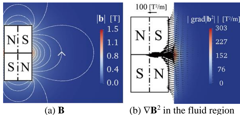
Fig. 10 Magnetic field and magnetic force of two block magnets.
