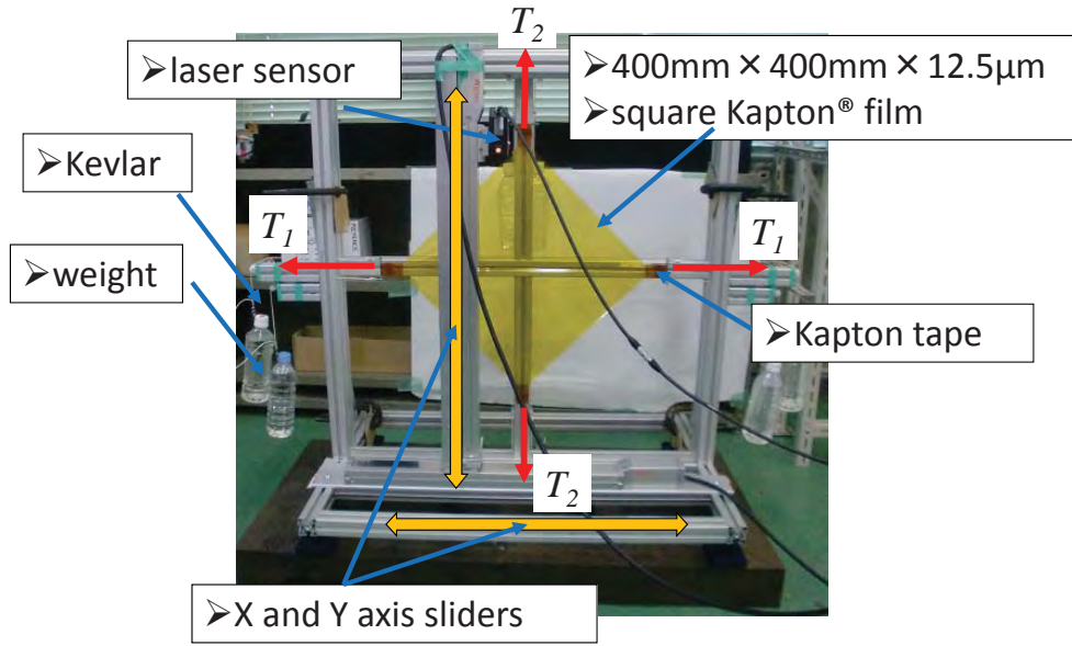
Figure 2. Experimental setup for wrinkle/slack control experiments.
