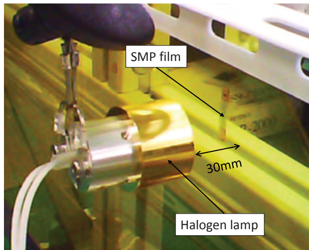
Figure 4. Photograph of halogen lamp for heating the SMP film.
