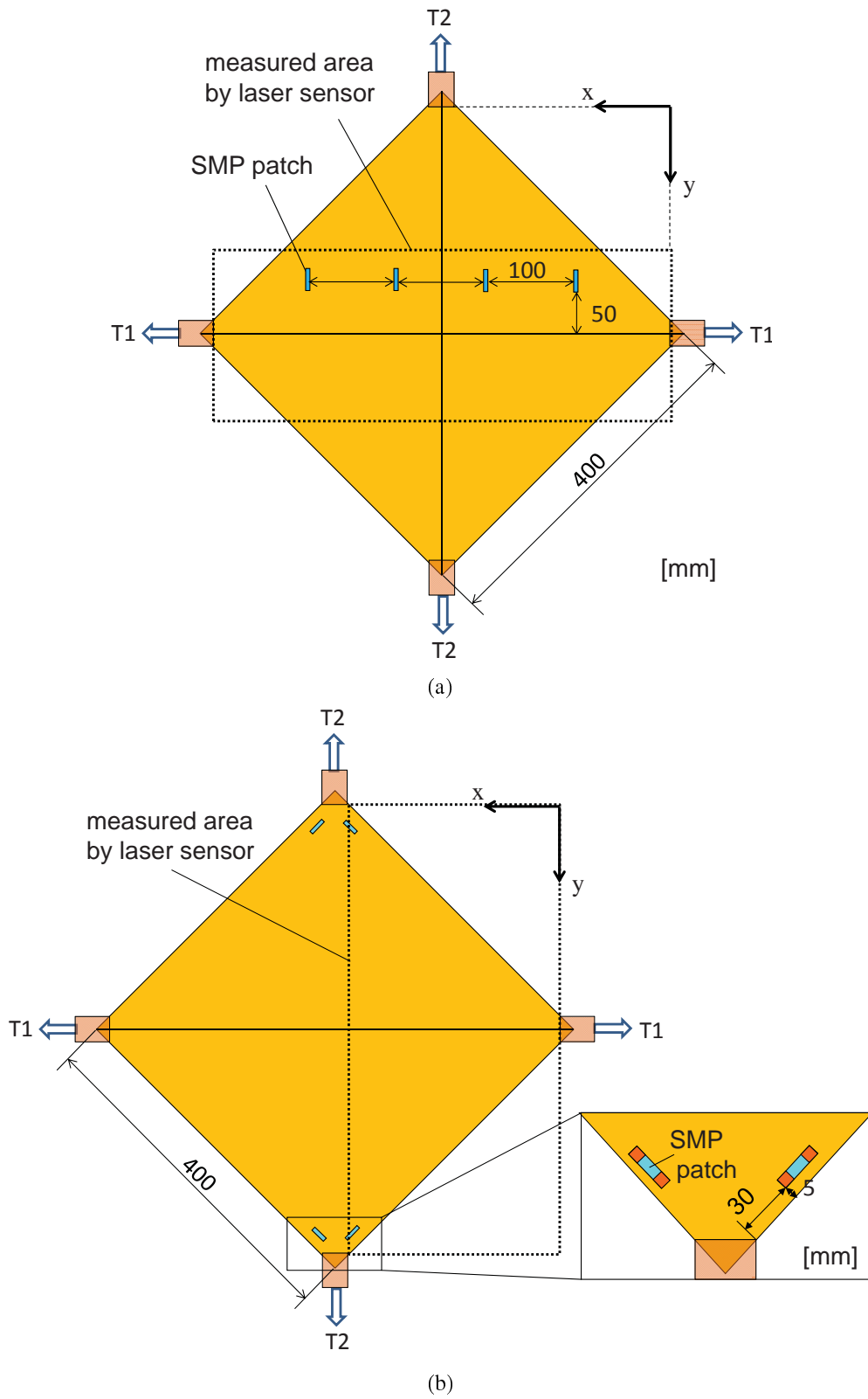
Figure 3. Square membrane subject to tensile forces T_1 = 9.54 [N] and T_2 = 1.74 [N] and the locations of the four SMP films: (a) for a wrinkle control experiment; (b) for a slack control experiment.
