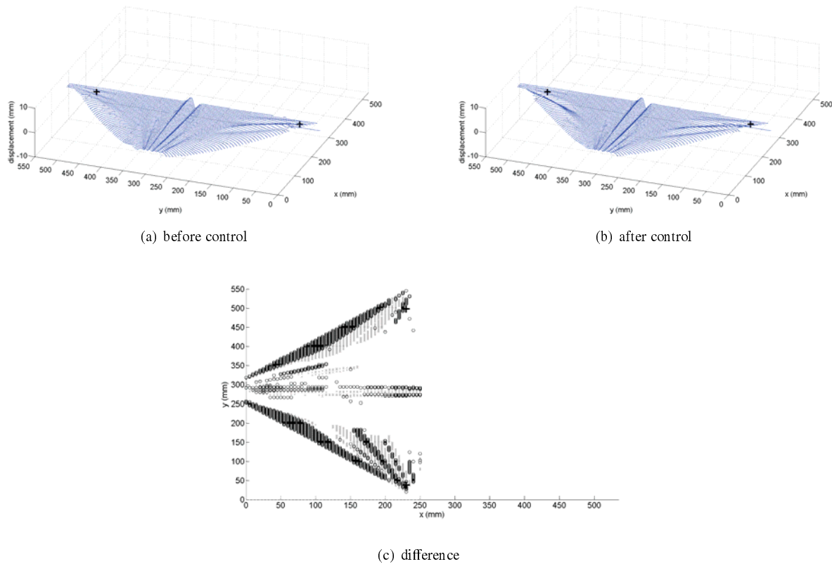
Figure 8. Comparison of measured out-of-plane displacement before and after slack control by SMP.
