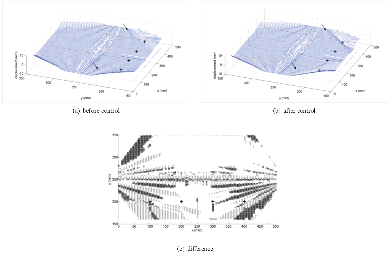
Figure 6. Comparison of measured out-of-plane displacement before and after wrinkle control by SMP.
