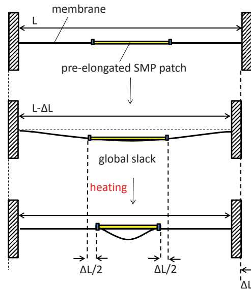
Figure 1. Concept of the shape control by SMP film on the membrane surface.
