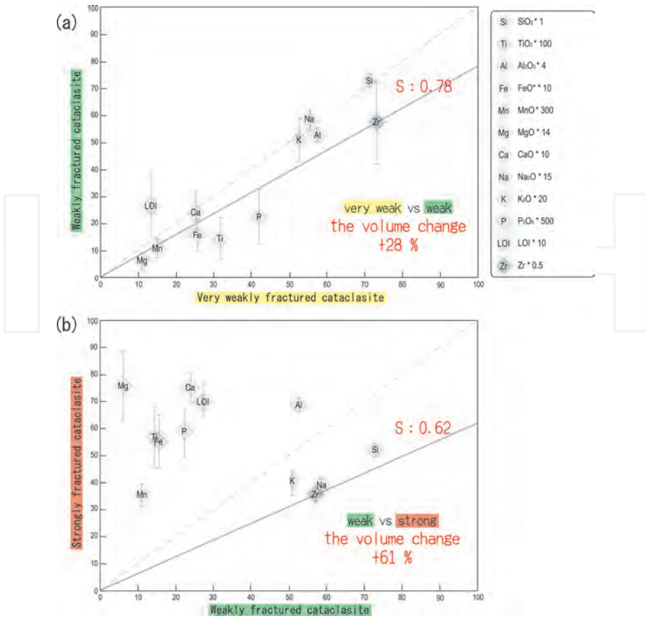
Figure 9. Isocon diagram for the Group 1 cataclasis samples with different degree of cataclasis. (a) Very weakly versus weakly fractured, and (b) weakly versus strongly fractured samples. The isocon diagram for weakly versus moderately fractured samples is not shown.
